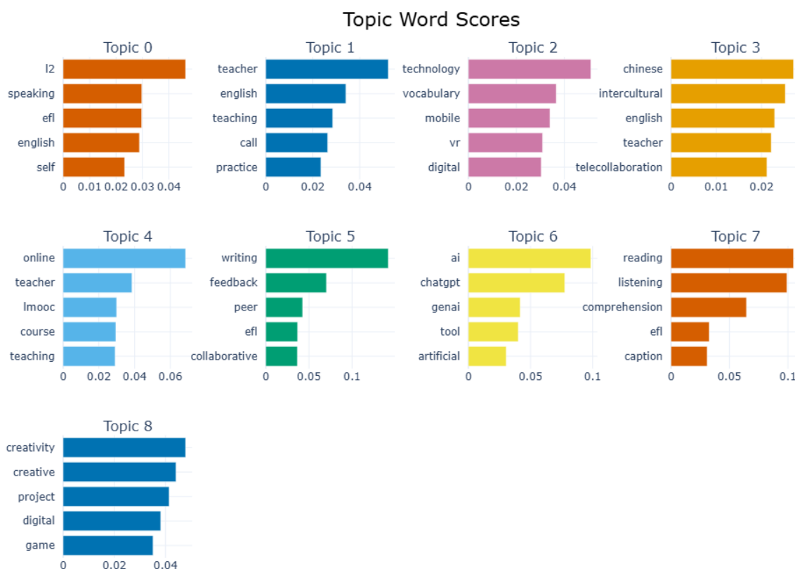
Figure 3. The core keywords for each topic and their c-TF-IDF scores
